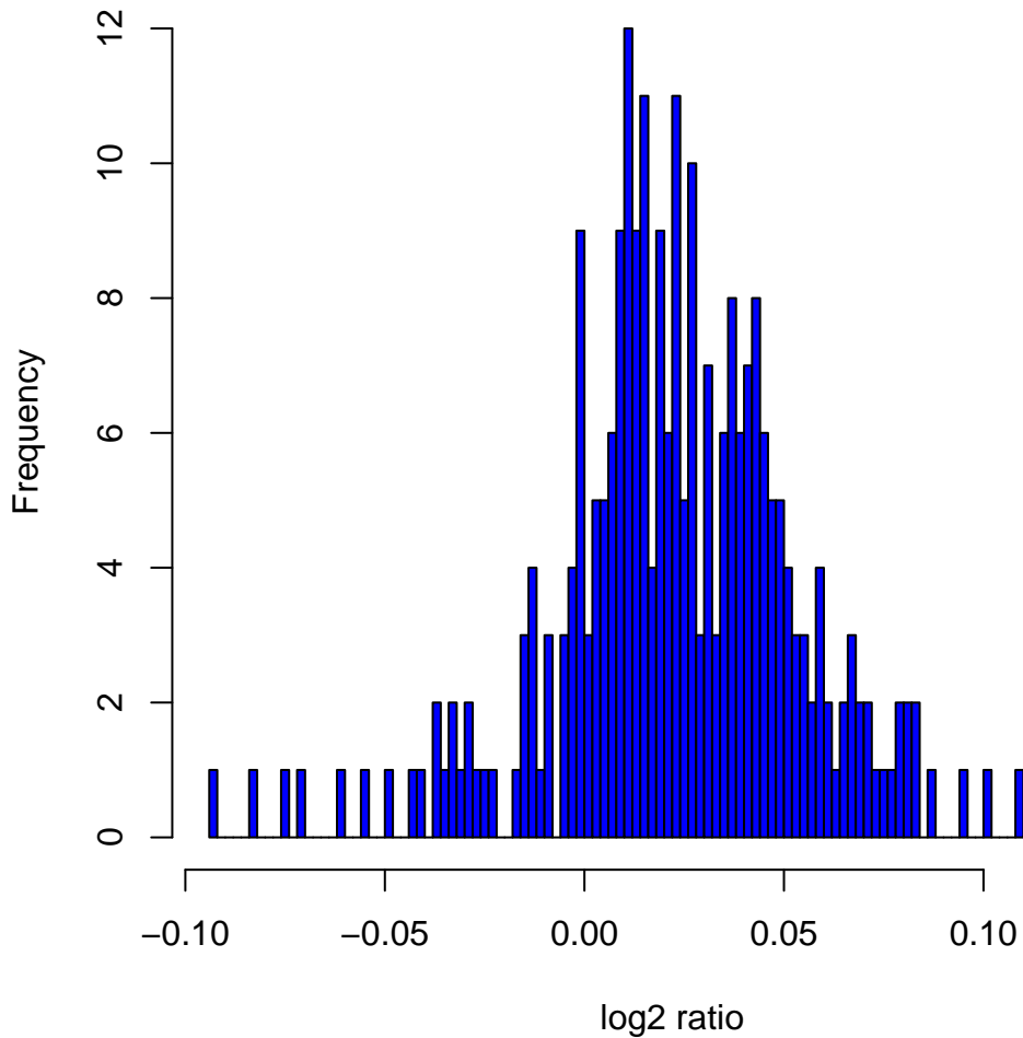
Histogram of log 2 ratios in 270 HapMap samples at clone Chr2tp-13C8
