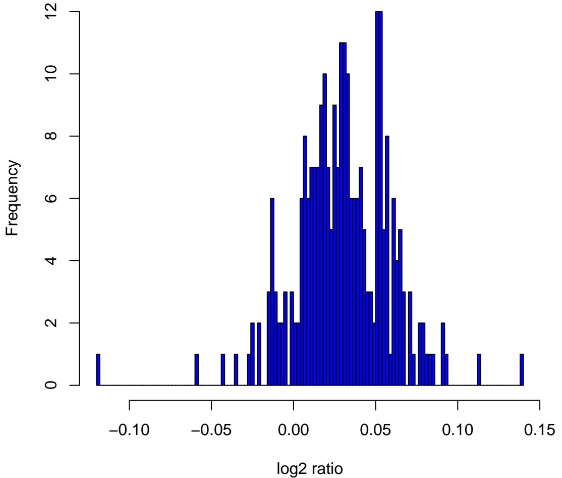
Histogram of log 2 ratios in 270 HapMap samples at clone Chr2tp-13D6
