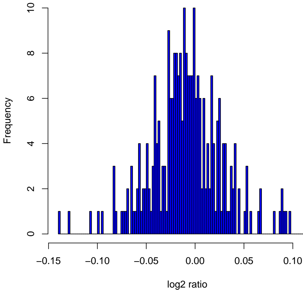
Histogram of log2ratios in 270 HapMap samples at clone Chr2tp-13G3
