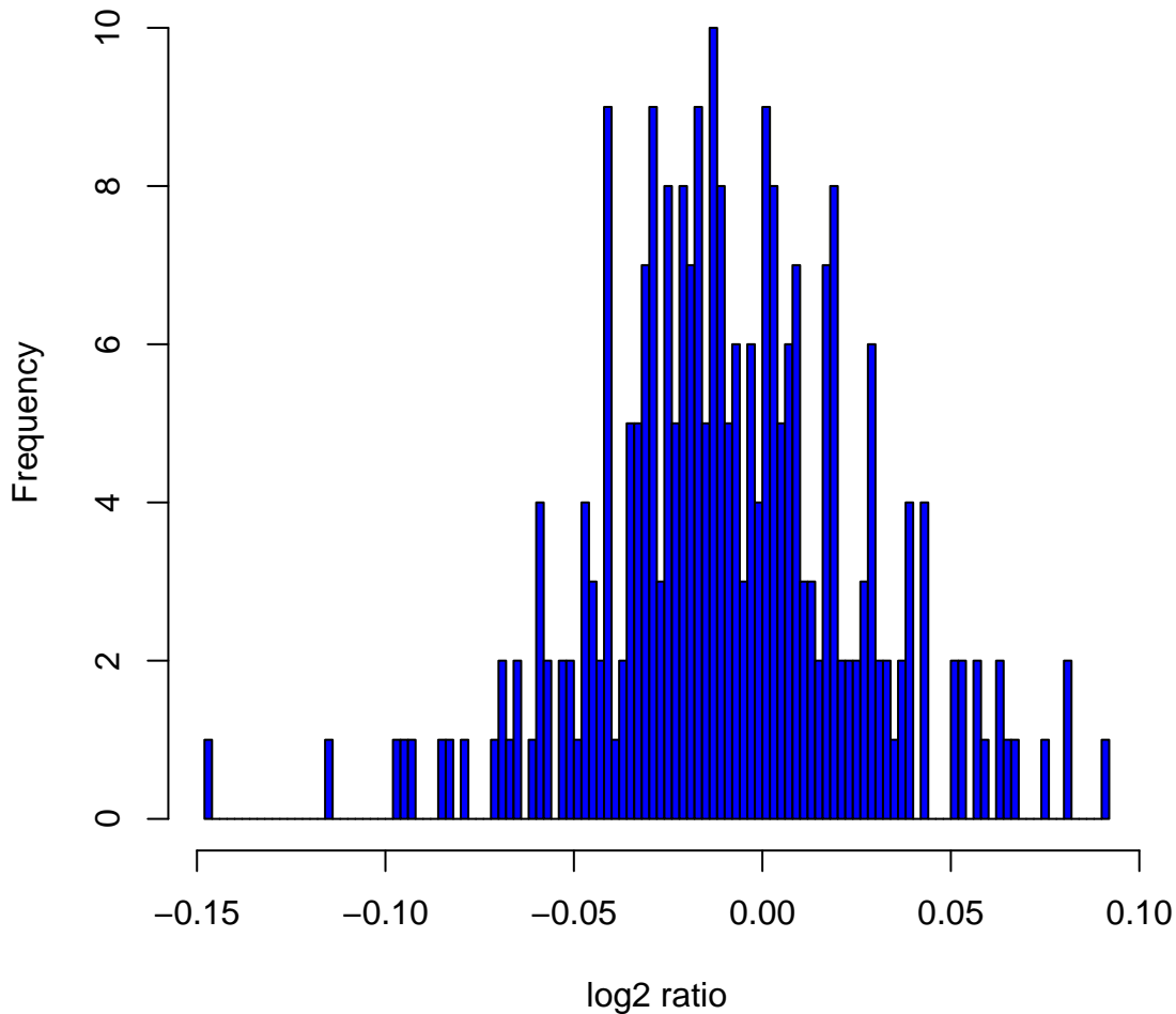
Histogram of log 2 ratios in 270 HapMap samples at clone Chr2tp-13G6
