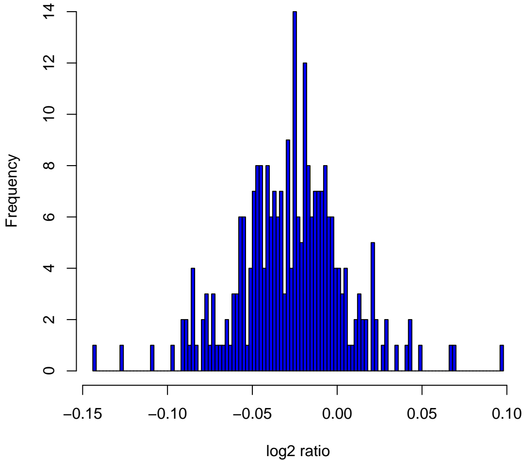
Histogram of log2ratios in 270 HapMap samples at clone Chr2tp-13H11
