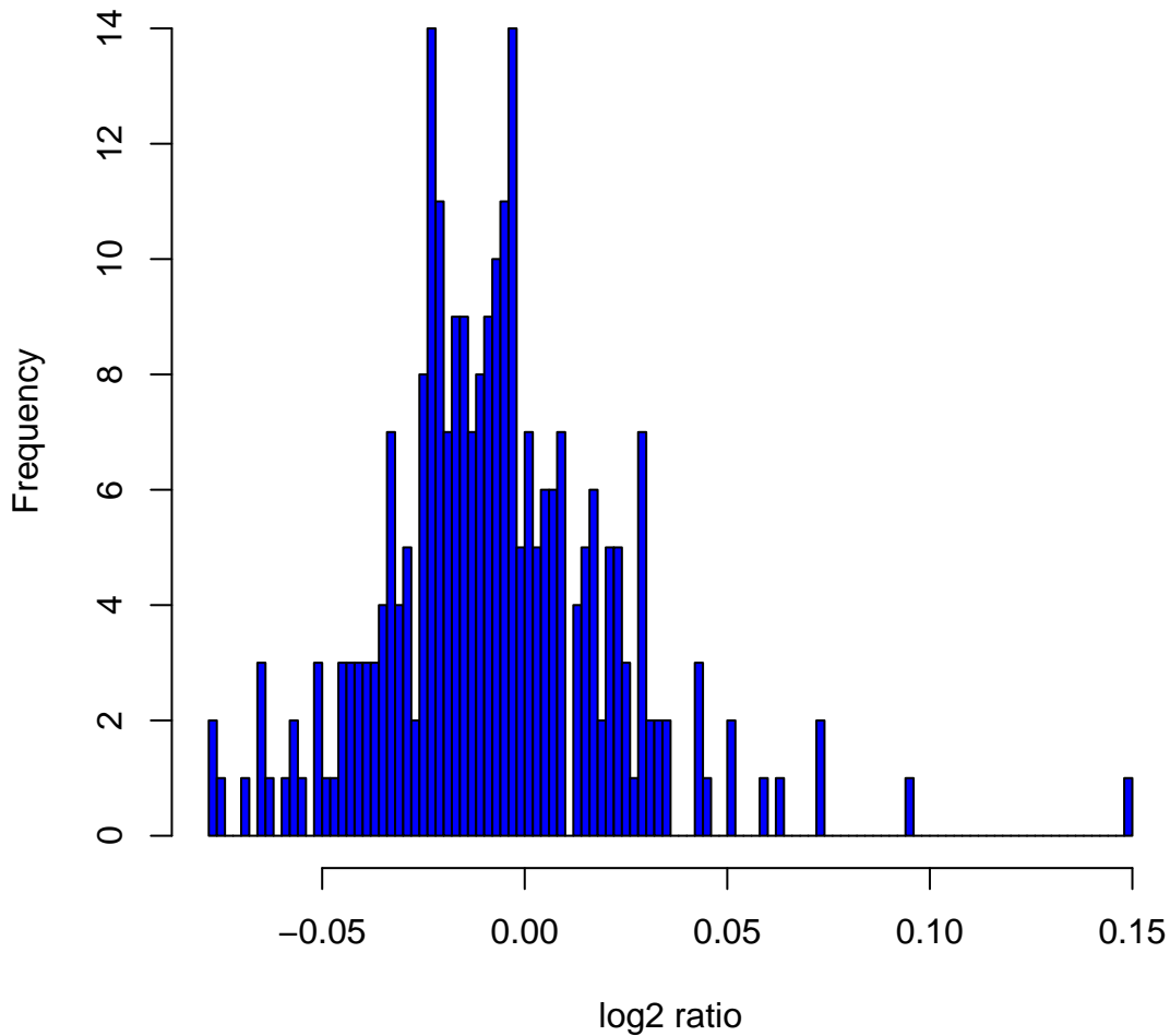
Histogram of log 2 ratios in 270 HapMap samples at clone Chr2tp-16B1
