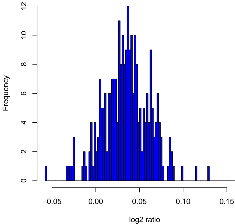
Histogram of log 2 ratios in 270 HapMap samples at clone Chr2tp-17A9
