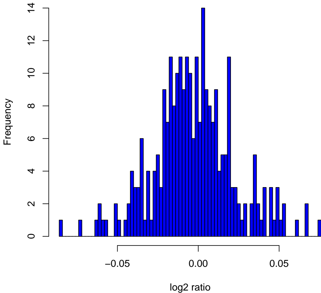
Histogram of log2ratios in 270 HapMap samples at clone Chr2tp-17C10
