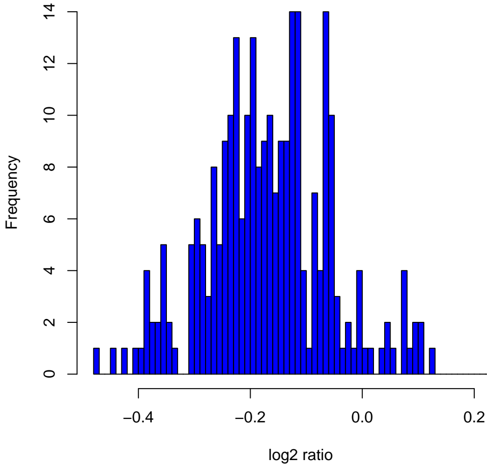
Histogram of log 2 ratios in 270 HapMap samples at clone Chr2tp-17C6
