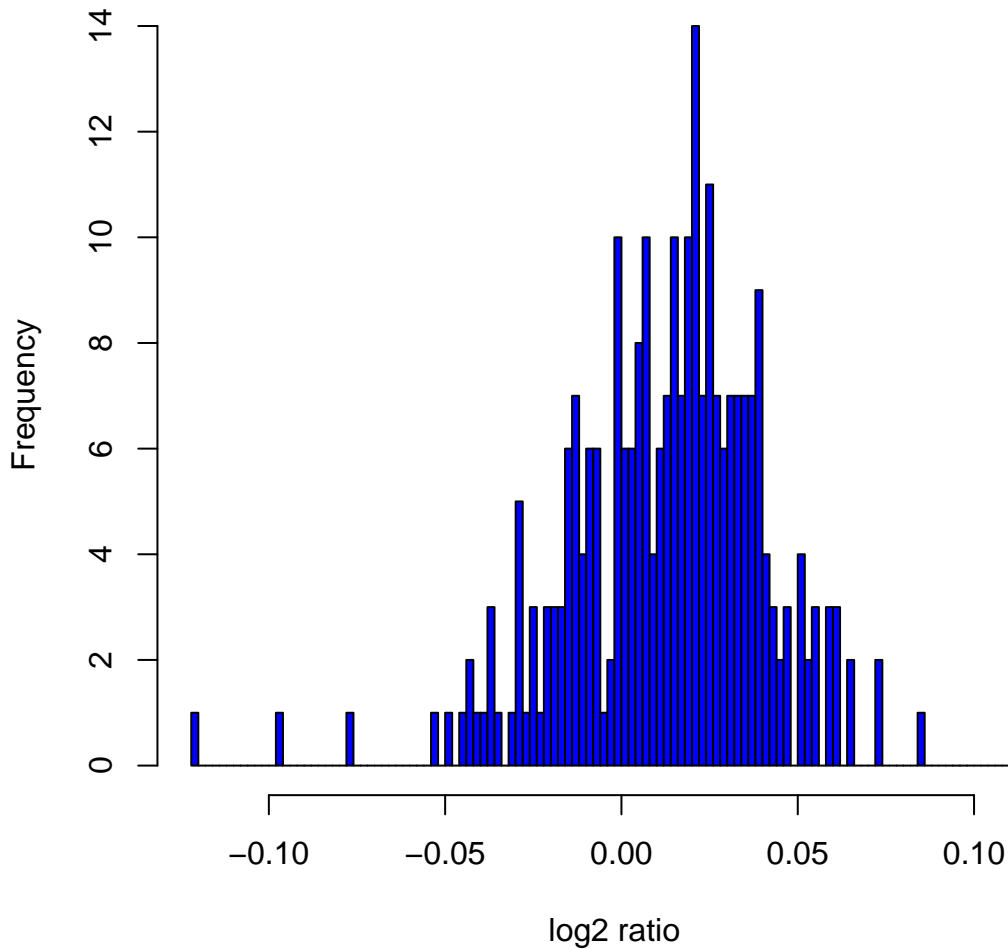
Histogram of log2ratios in 270 HapMap samples at clone Chr2tp-17D12
