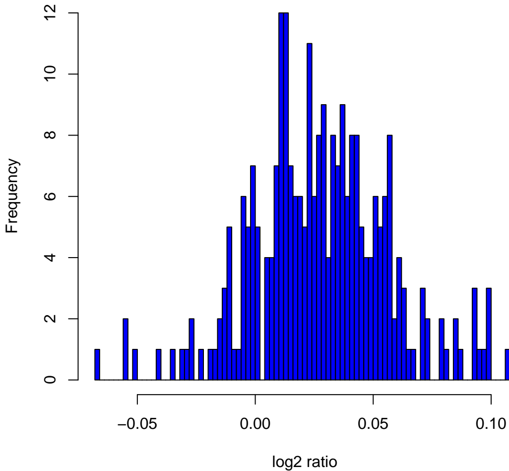
Histogram of log 2 ratios in 270 HapMap samples at clone Chr2tp-17H3
