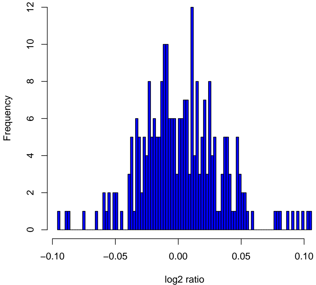
Histogram of log2ratios in 270 HapMap samples at clone Chr2tp-18A11
