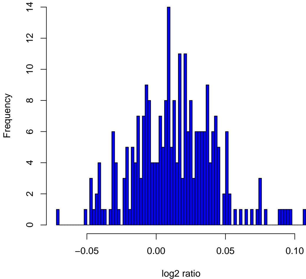
Histogram of log2ratios in 270 HapMap samples at clone Chr2tp-18D11
