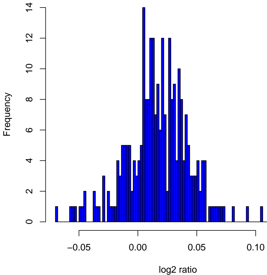
Histogram of log 2 ratios in 270 HapMap samples at clone Chr2tp-18D4
