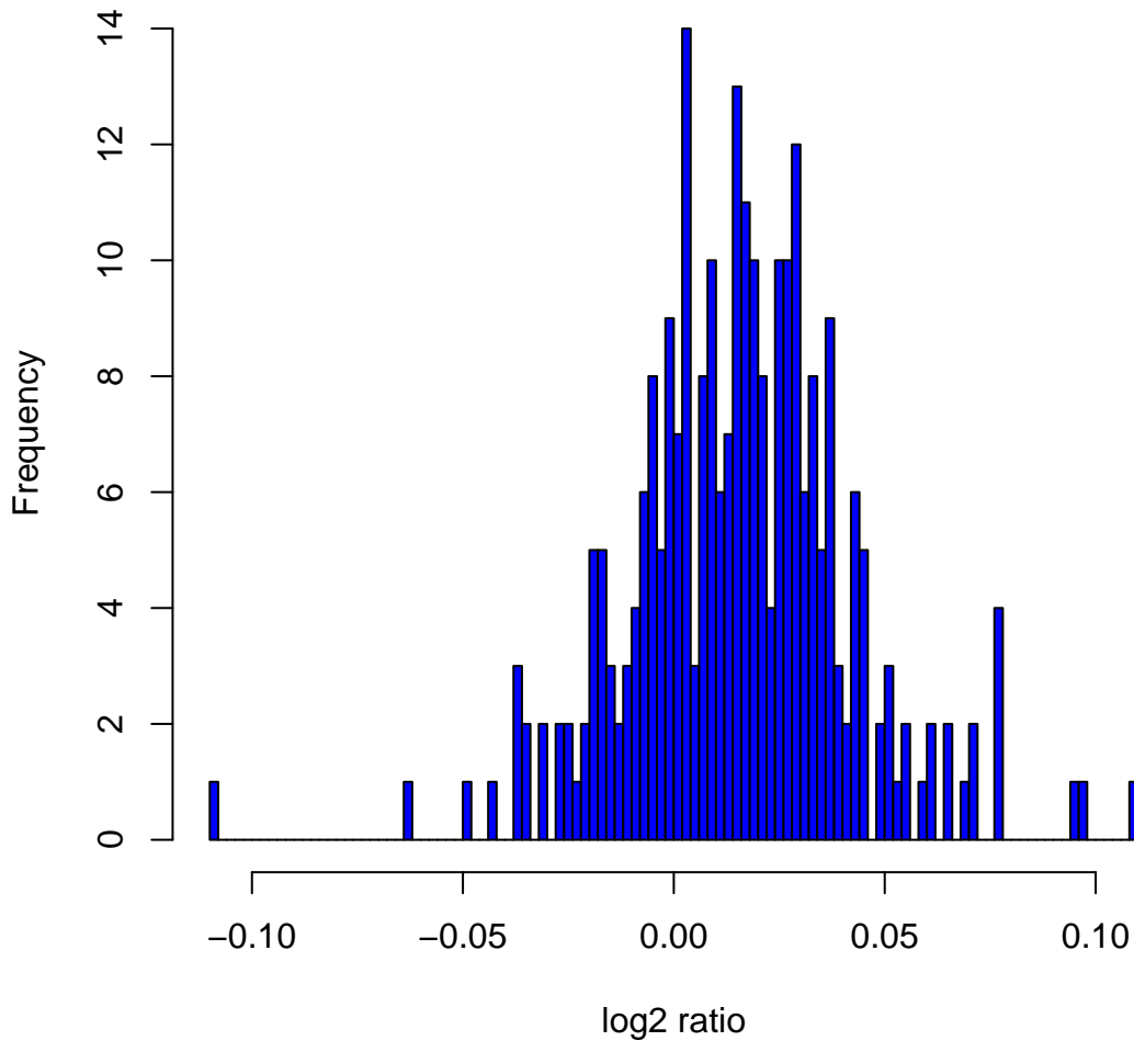
Histogram of log 2 ratios in 270 HapMap samples at clone Chr2tp-18G1
