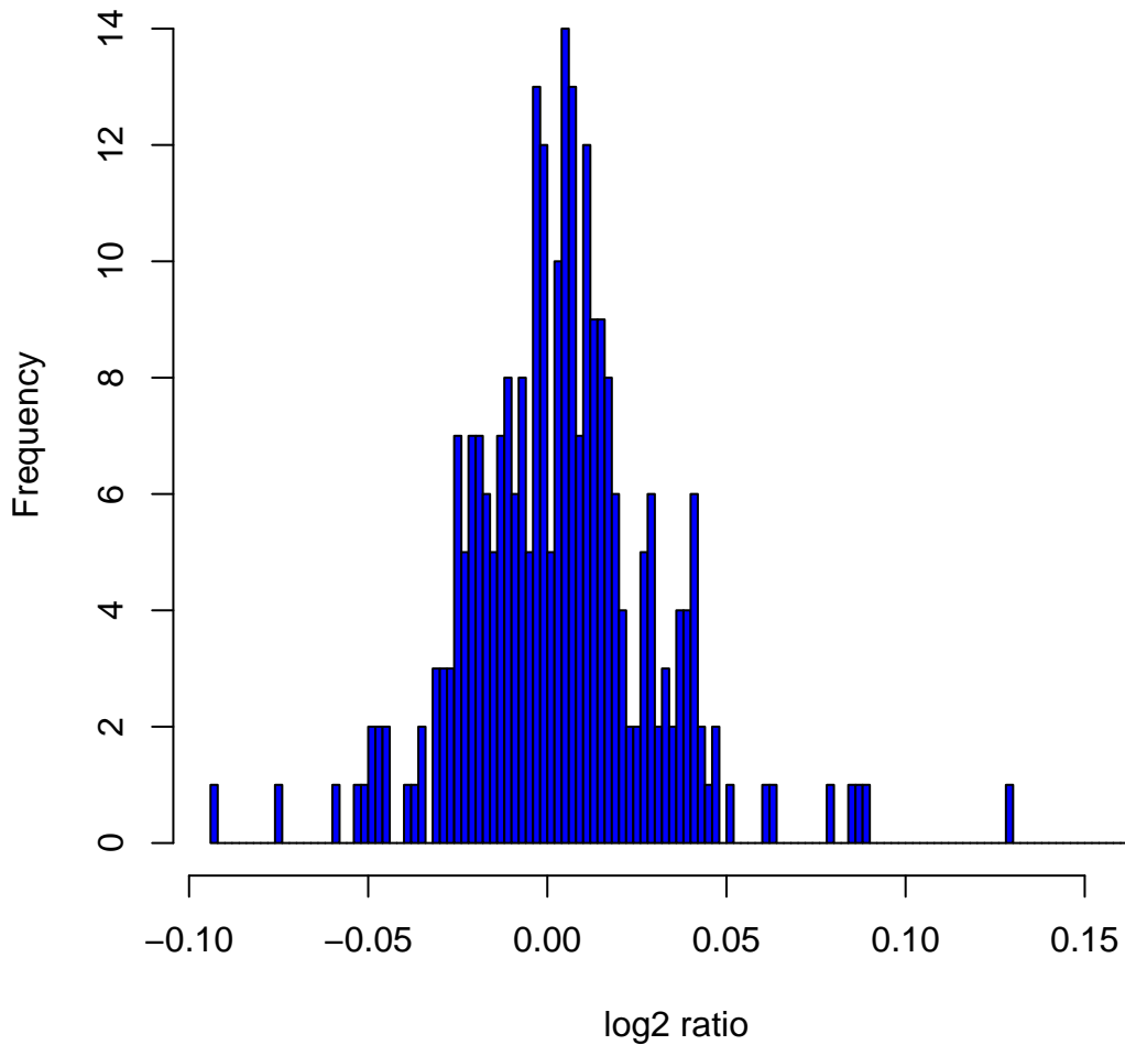
Histogram of \log_2 ratios in 270 HapMap samples at clone Chr2tp-18G3
