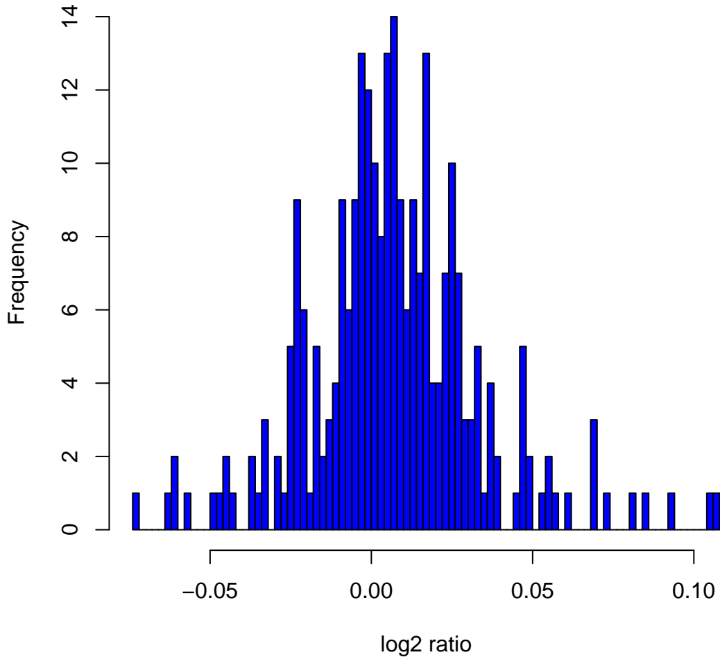
Histogram of log 2 ratios in 270 HapMap samples at clone Chr2tp-18G7
