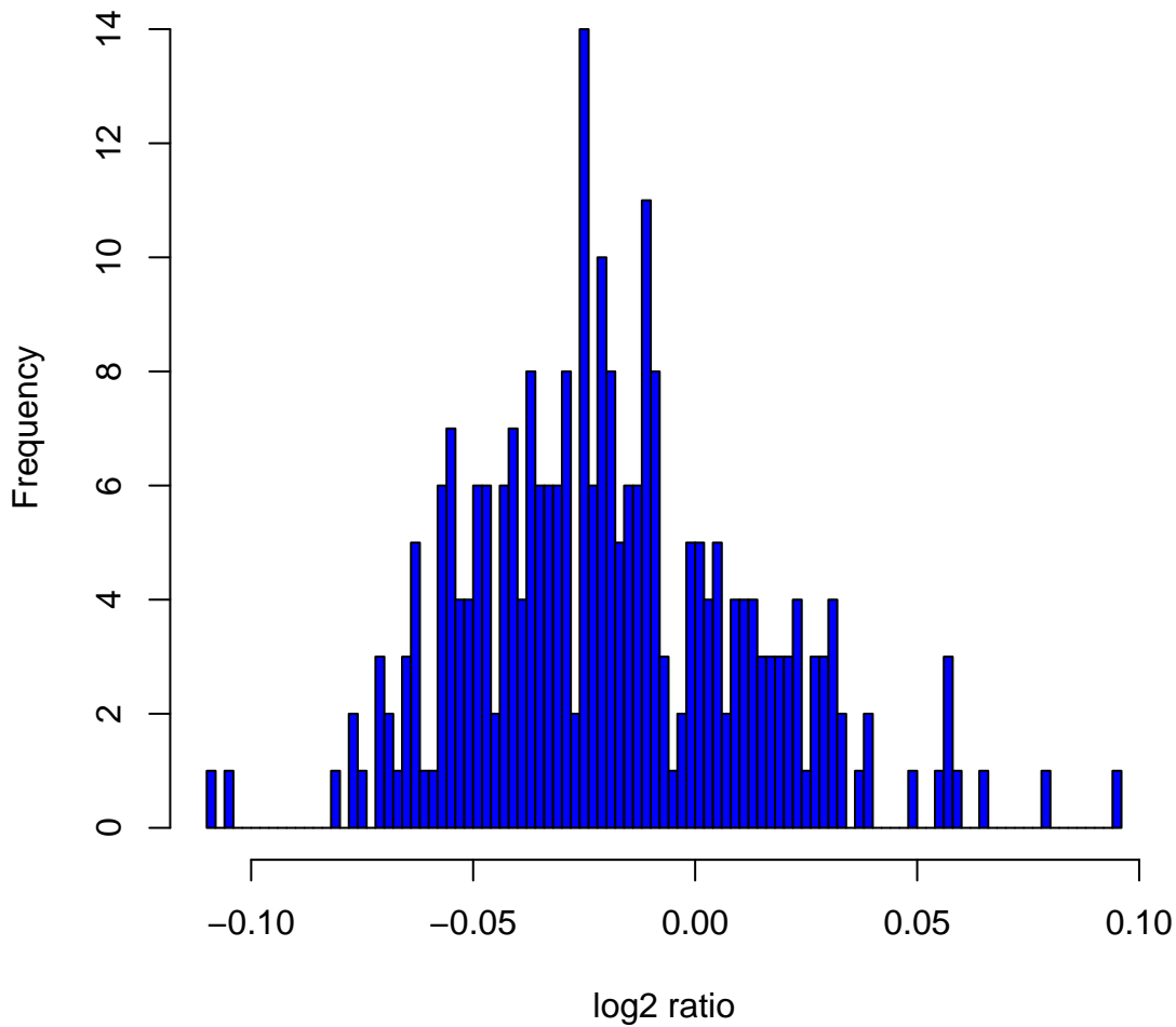
Histogram of log 2 ratios in 270 HapMap samples at clone Chr2tp-18H9
