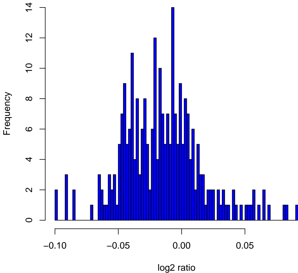
Histogram of \log_2 ratios in 270 HapMap samples at clone Chr2tp-19A2
