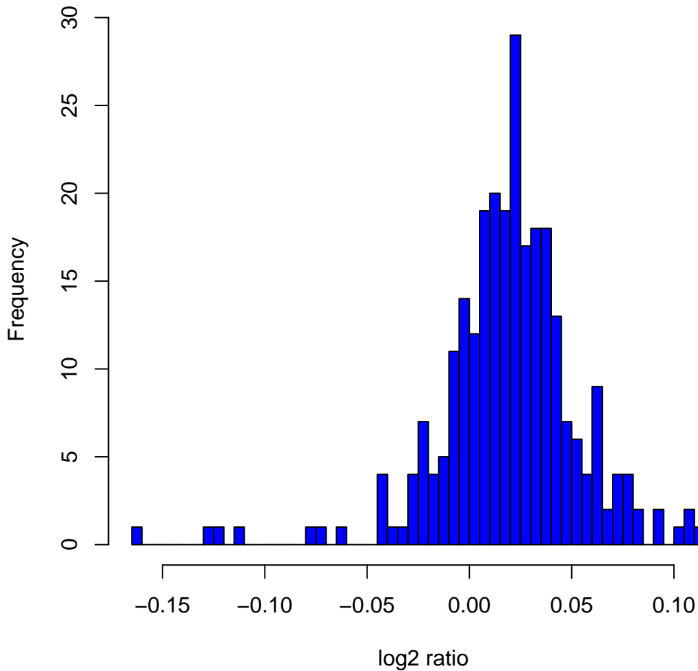
Histogram of log 2 ratios in 270 HapMap samples at clone Chr2tp-19A4
