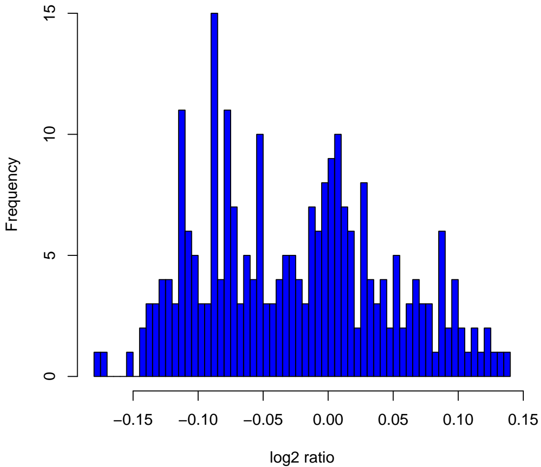
Histogram of log2ratios in 270 HapMap samples at clone Chr2tp-19H6
