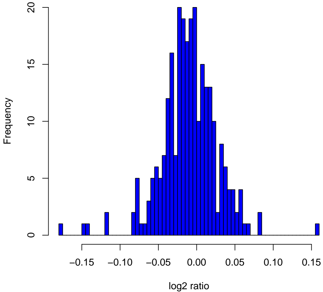
Histogram of log 2 ratios in 270 HapMap samples at clone Chr2tp-1A12
