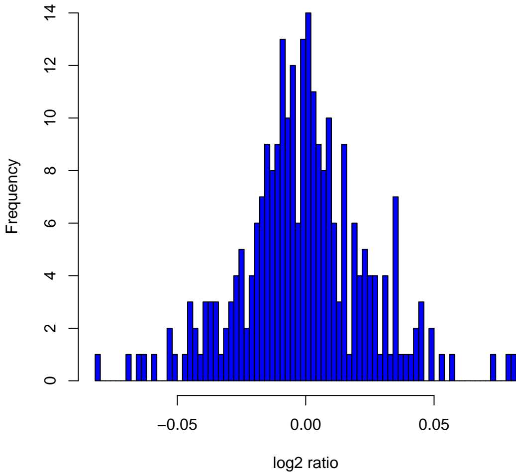
Histogram of \log_2 ratios in 270 HapMap samples at clone Chr2tp-1A8
