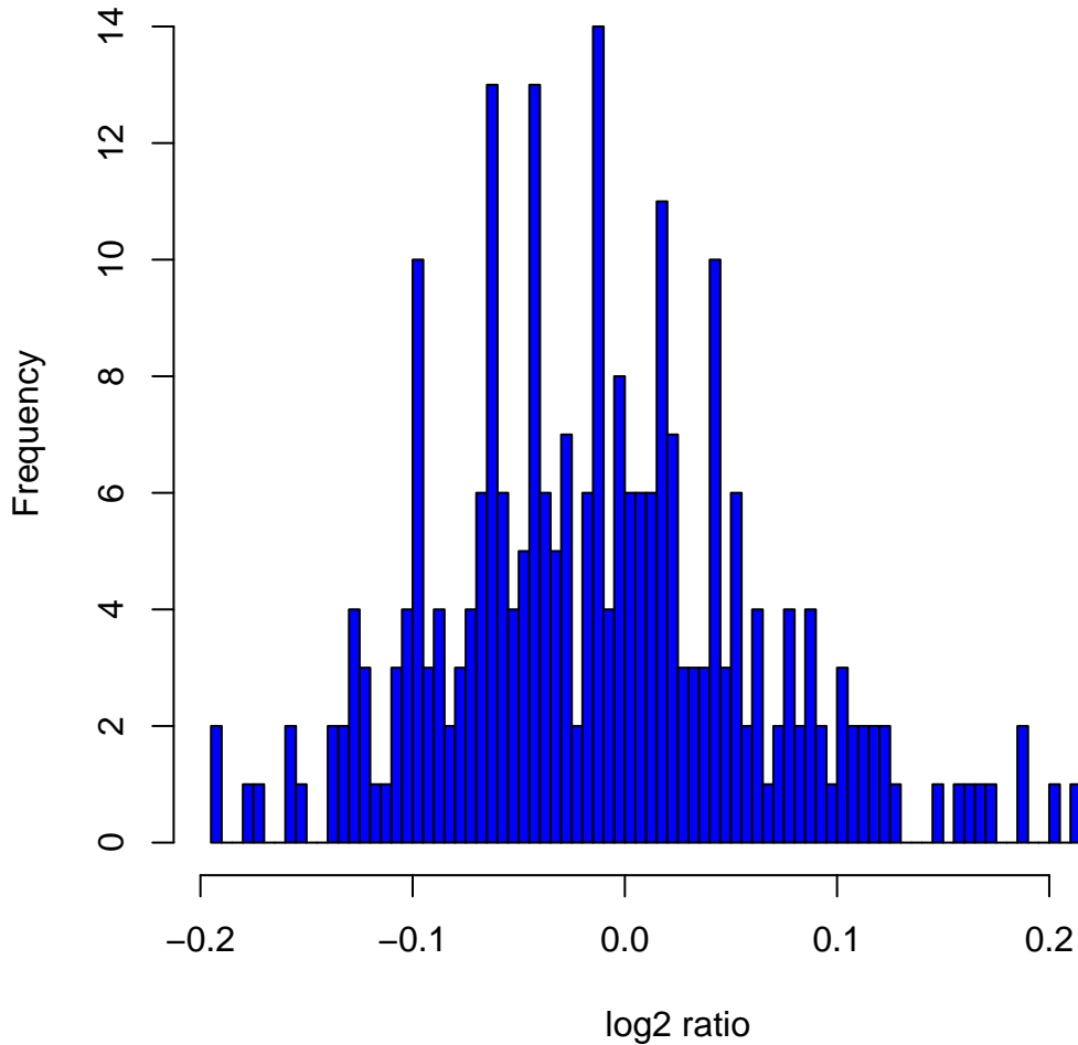
Histogram of \log_2 ratios in 270 HapMap samples at clone Chr2tp-1B10
