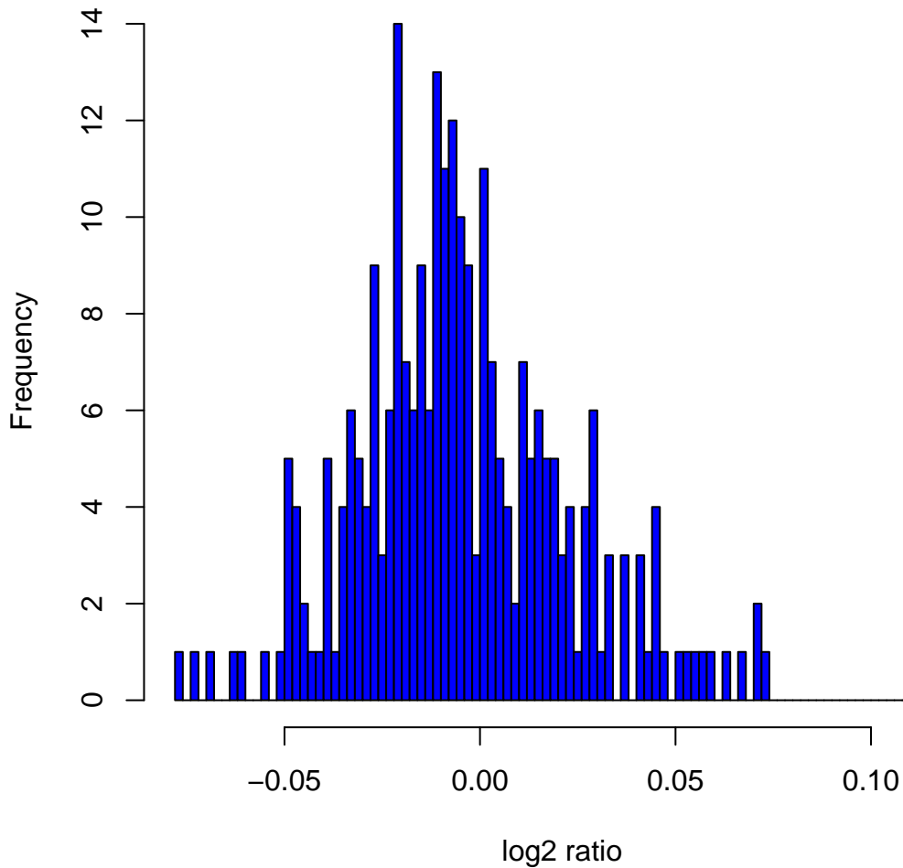
Histogram of \log_2 ratios in 270 HapMap samples at clone Chr2tp-1B9
