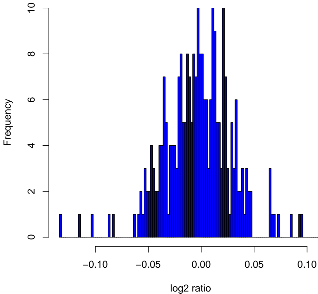
Histogram of \log_2 ratios in 270 HapMap samples at clone Chr2tp-1D1
