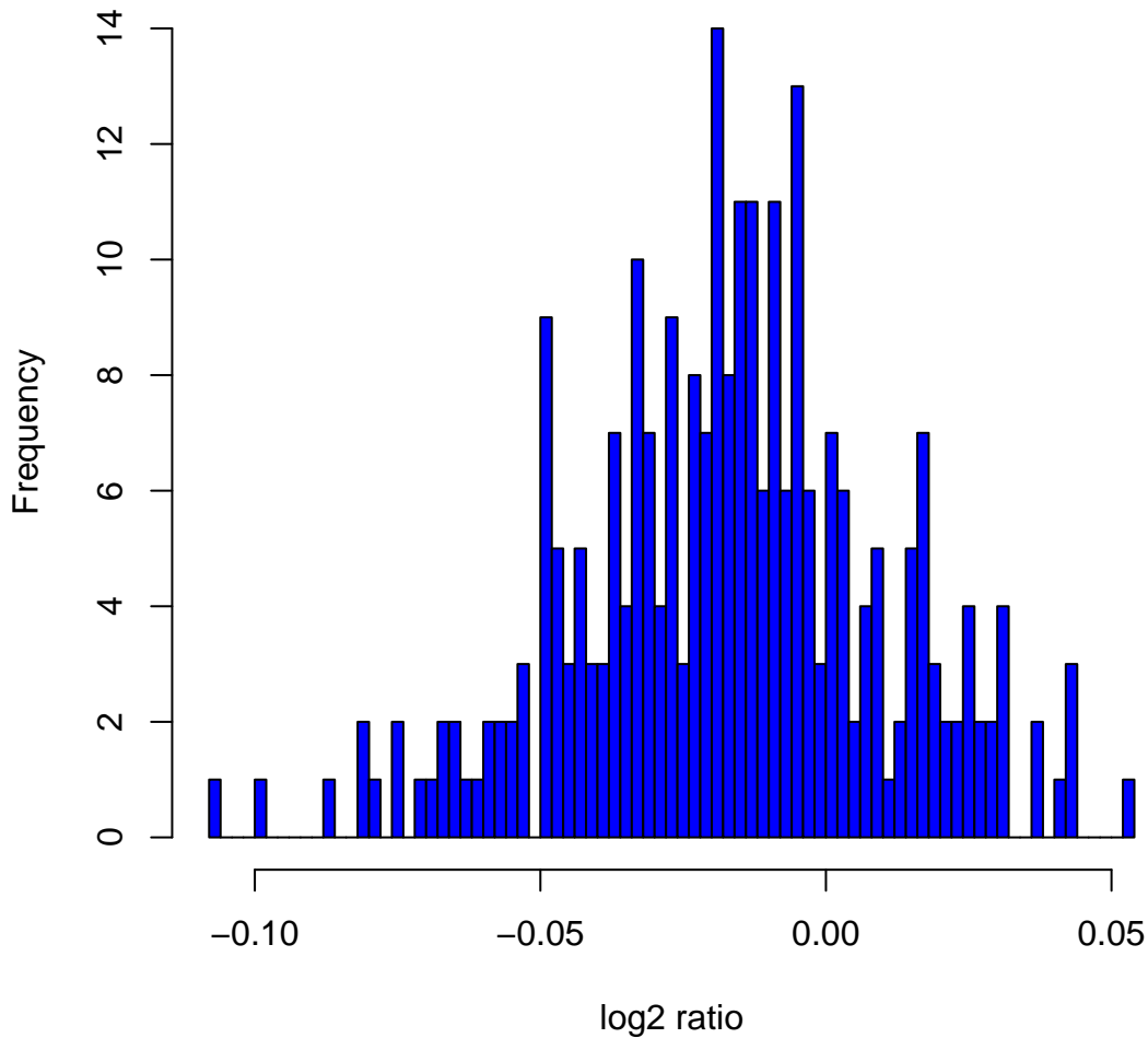
Histogram of log 2 ratios in 270 HapMap samples at clone Chr2tp-1D5
