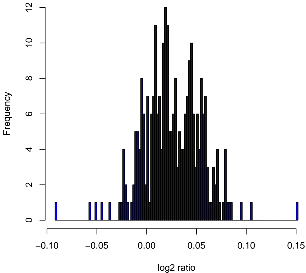
Histogram of \log_2 ratios in 270 HapMap samples at clone Chr2tp-1D6
