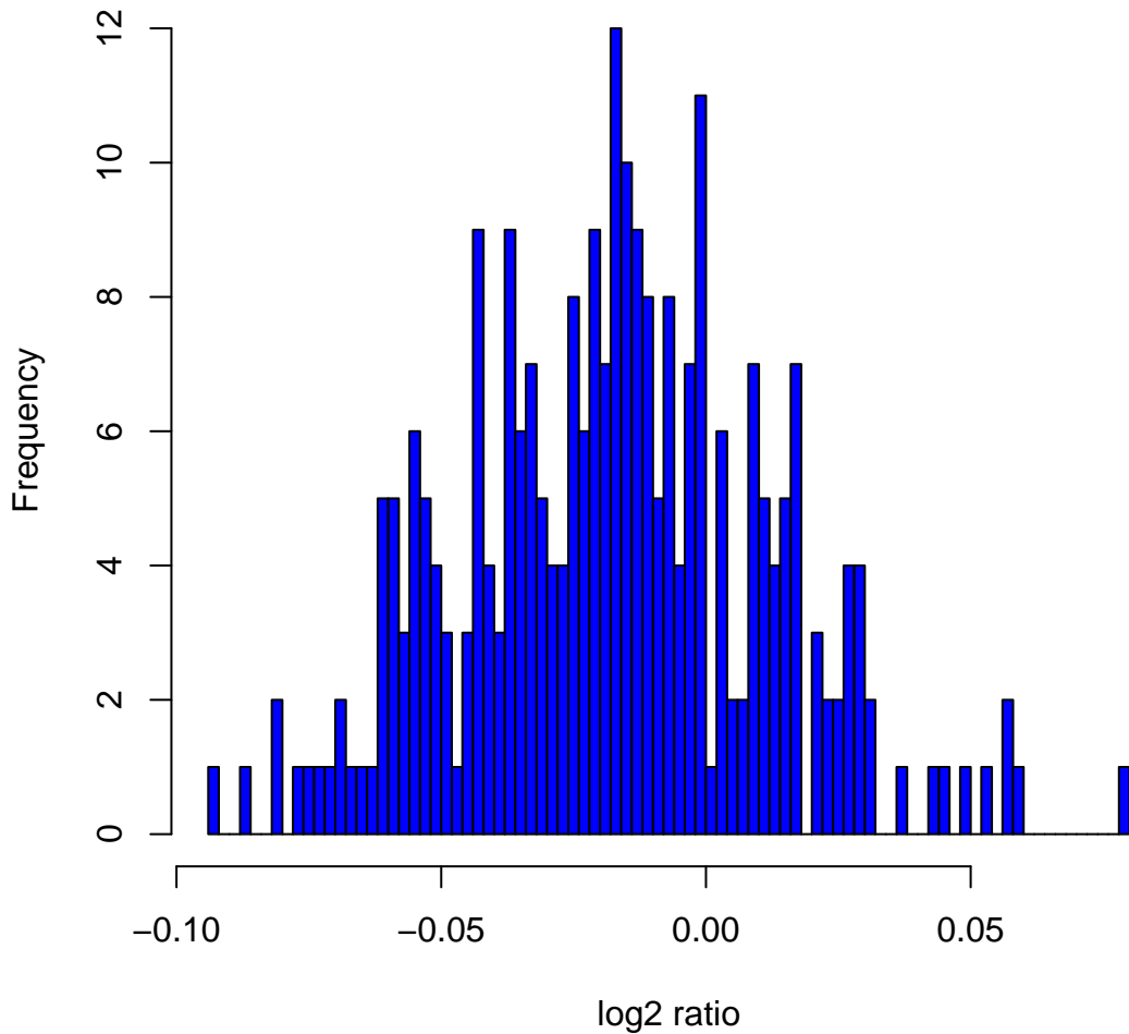
Histogram of \log_2 ratios in 270 HapMap samples at clone Chr2tp-1E5
