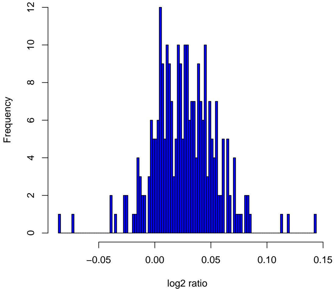
Histogram of log 2 ratios in 270 HapMap samples at clone Chr2tp-1F8
