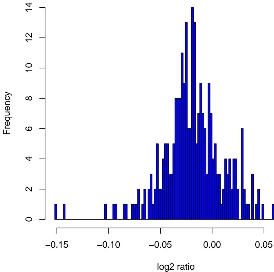
Histogram of log 2 ratios in 270 HapMap samples at clone Chr2tp-1G11
