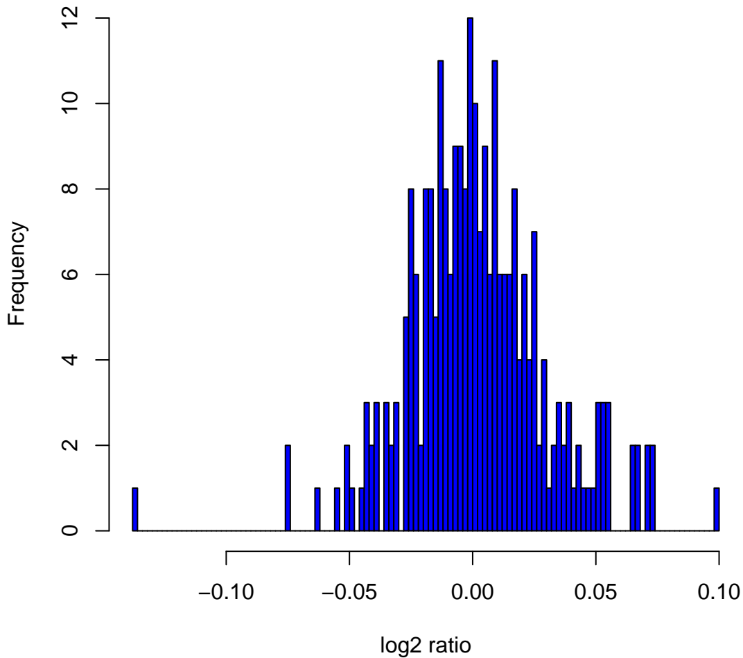
Histogram of log2ratios in 270 HapMap samples at clone Chr2tp-20A12
