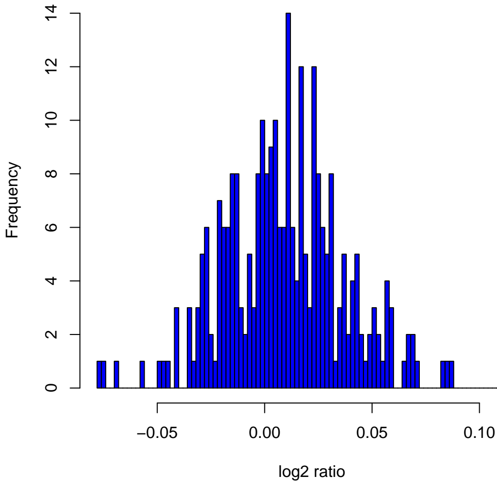
Histogram of log2ratios in 270 HapMap samples at clone Chr2tp-20B11
