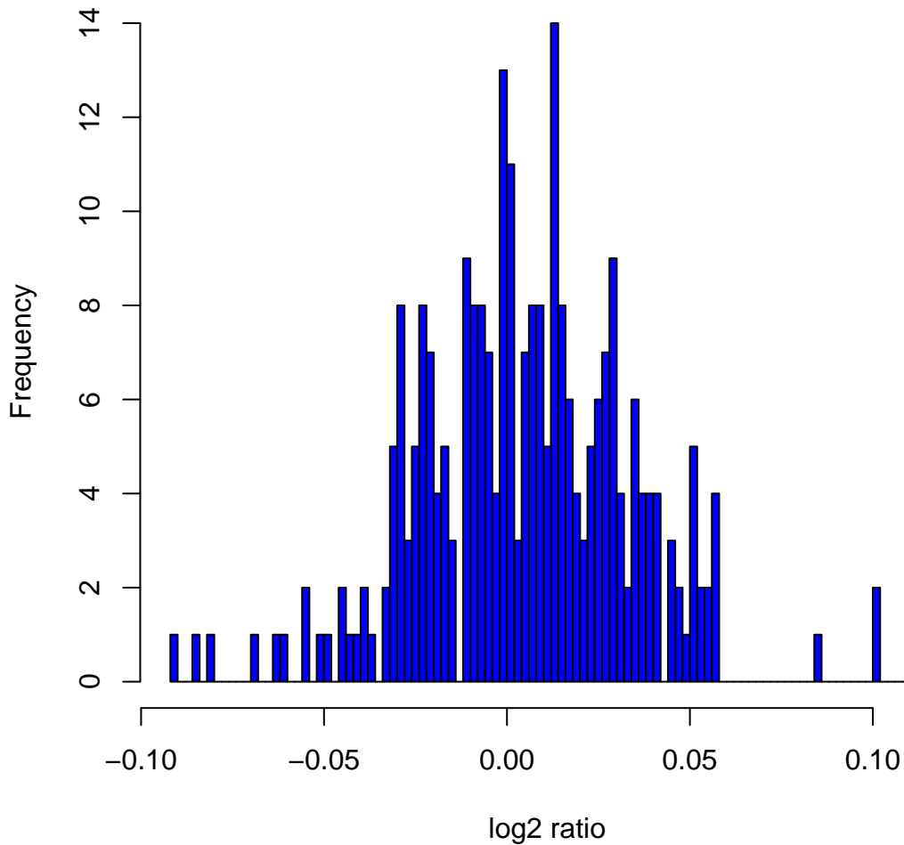
Histogram of log2ratios in 270 HapMap samples at clone Chr2tp-20G2
