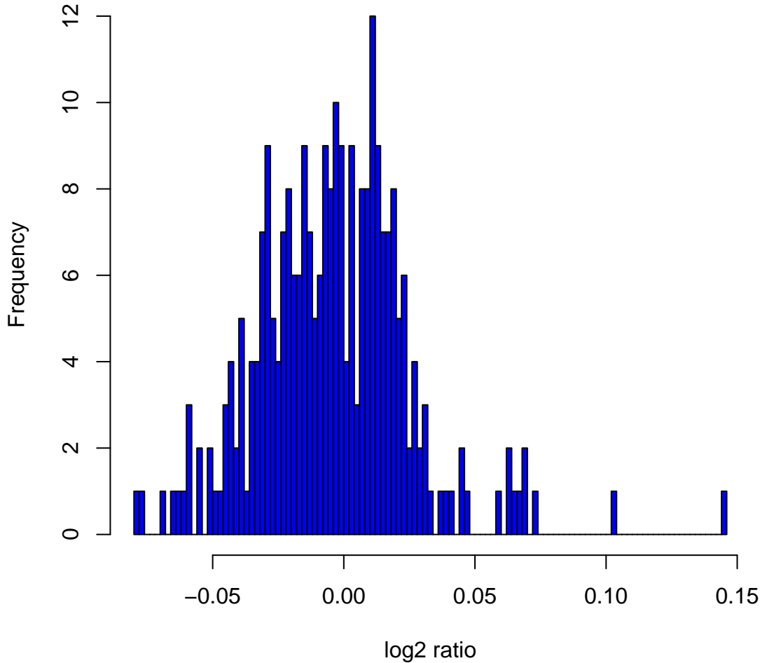
Histogram of log 2 ratios in 270 HapMap samples at clone Chr2tp-20G3
