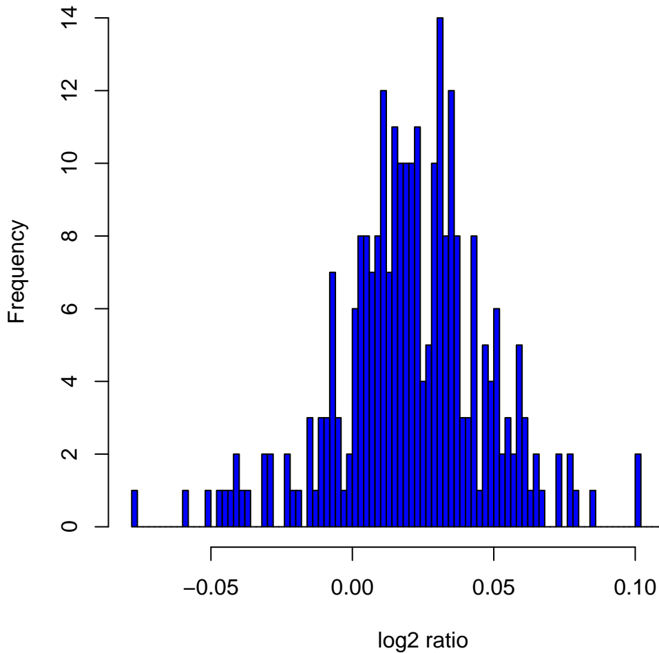
Histogram of \log_2 ratios in 270 HapMap samples at clone Chr2tp-20G5
