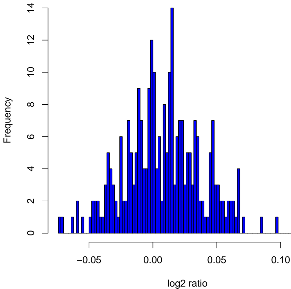
Histogram of log 2 ratios in 270 HapMap samples at clone Chr2tp-20H2
