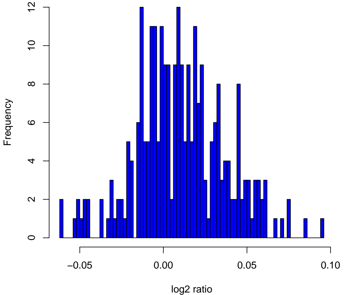
Histogram of log2ratios in 270 HapMap samples at clone Chr2tp-21A11
