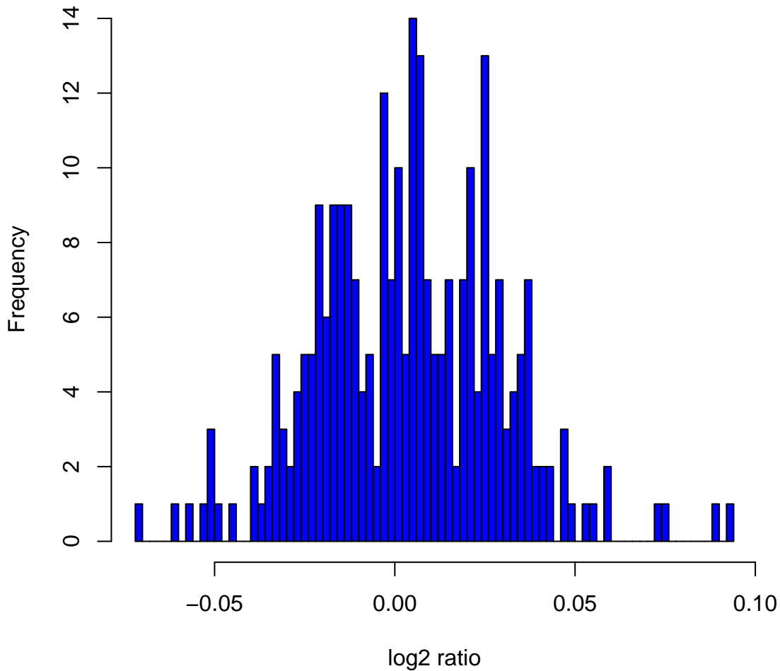
Histogram of log2ratios in 270 HapMap samples at clone Chr2tp-21B10
