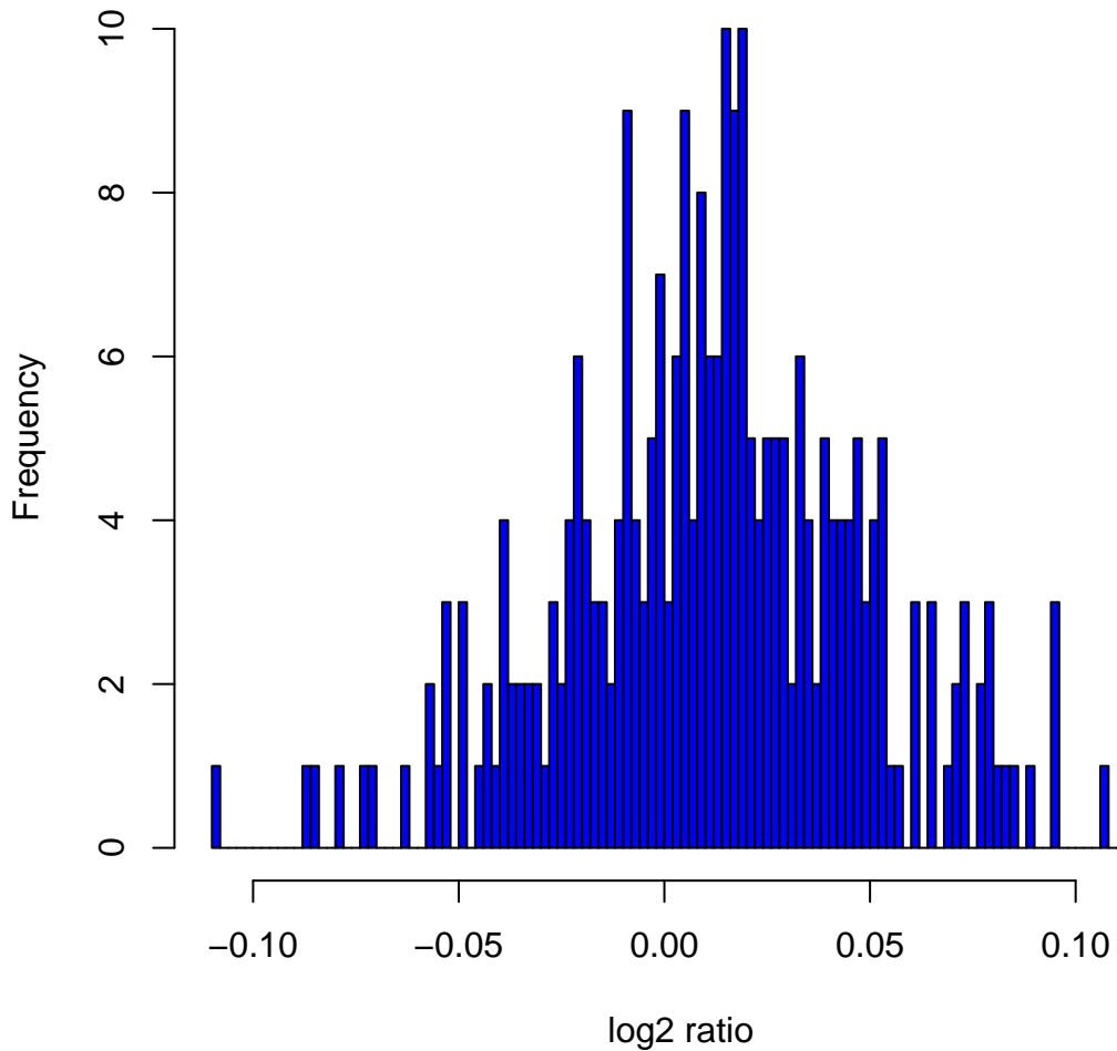
Histogram of \log_2 ratios in 270 HapMap samples at clone Chr2tp-21H1
