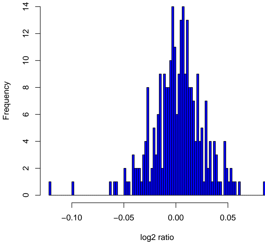
Histogram of log 2 ratios in 270 HapMap samples at clone Chr2tp-21H9
