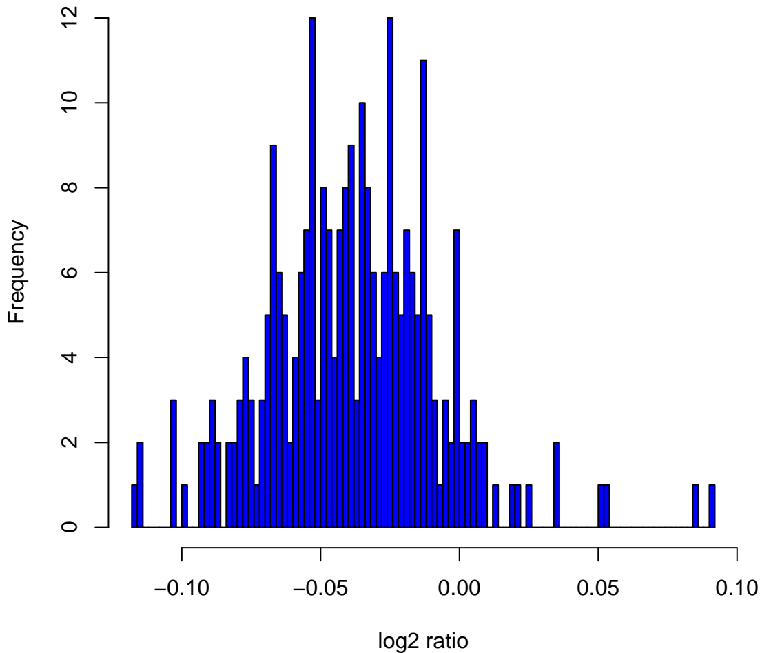
Histogram of log2ratios in 270 HapMap samples at clone Chr2tp-22A11
