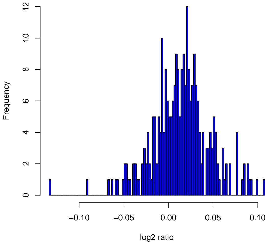
Histogram of log2ratios in 270 HapMap samples at clone Chr2tp-22A12
