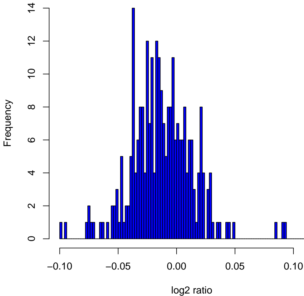
Histogram of log 2 ratios in 270 HapMap samples at clone Chr2tp-22C5
