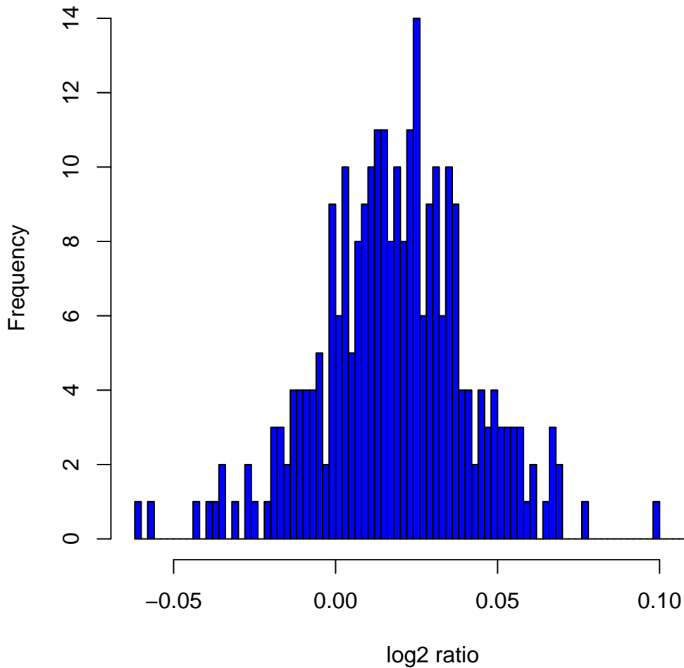
Histogram of log 2 ratios in 270 HapMap samples at clone Chr2tp-23A1
