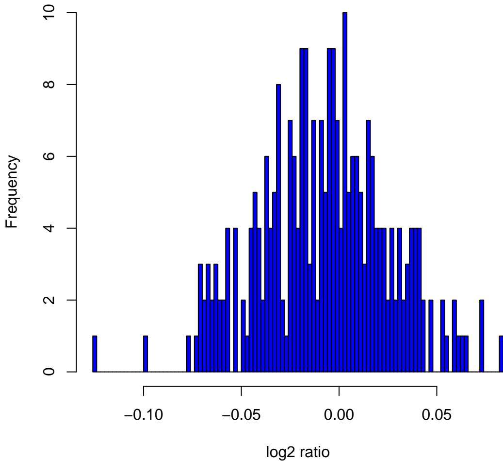
Histogram of log 2 ratios in 270 HapMap samples at clone Chr2tp-23C3
