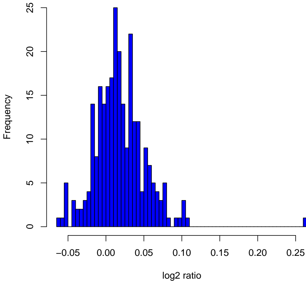
Histogram of log2ratios in 270 HapMap samples at clone Chr2tp-24D10
