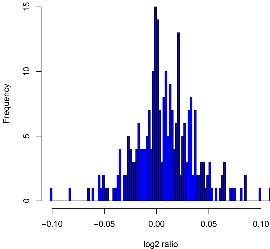
Histogram of log2ratios in 270 HapMap samples at clone Chr2tp-24D12
