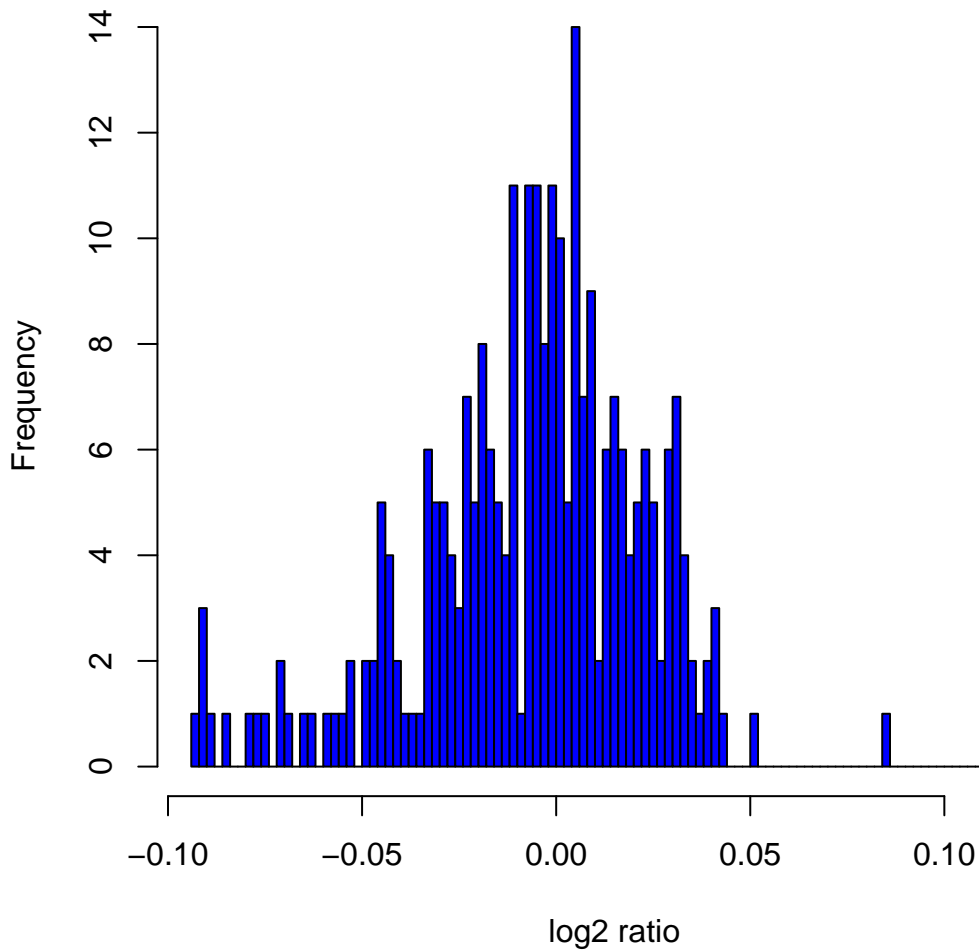
Histogram of log 2 ratios in 270 HapMap samples at clone Chr2tp-24E7
