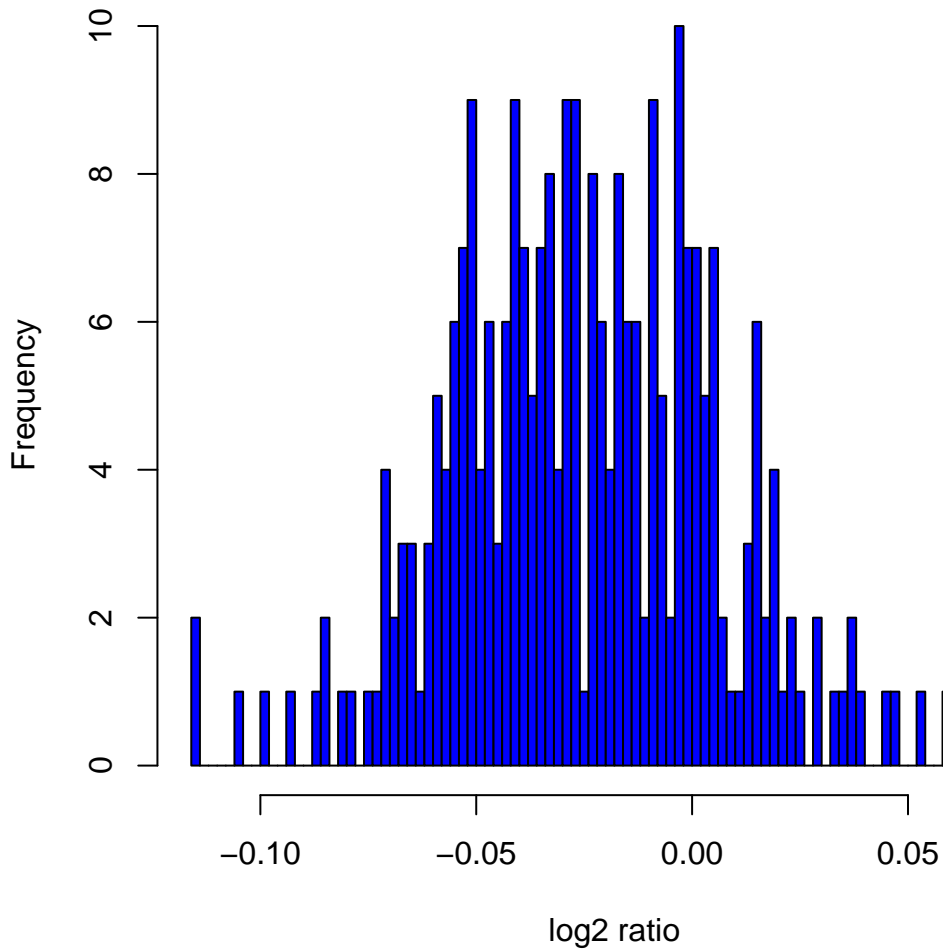
Histogram of \log_2 ratios in 270 HapMap samples at clone Chr2tp-24H10
